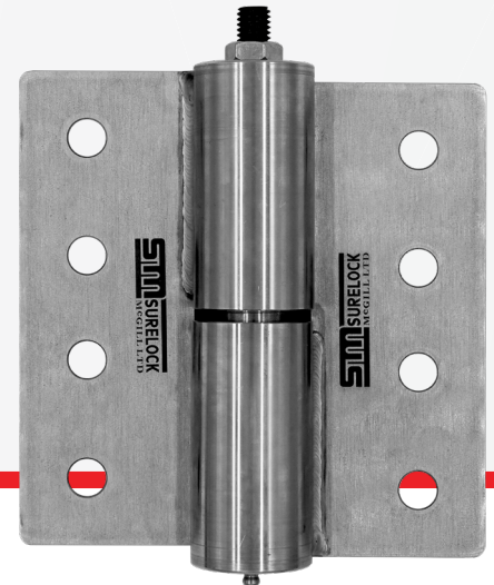
HC44 LEFT HAND CAM LIFT
