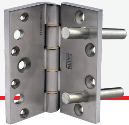
HA7 60 MM EXTENDED HIGH-PERFORMANCE HINGE WITH OPTIONAL SCREW-IN PIN
