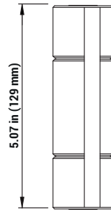
HT10 SIDE VIEW
