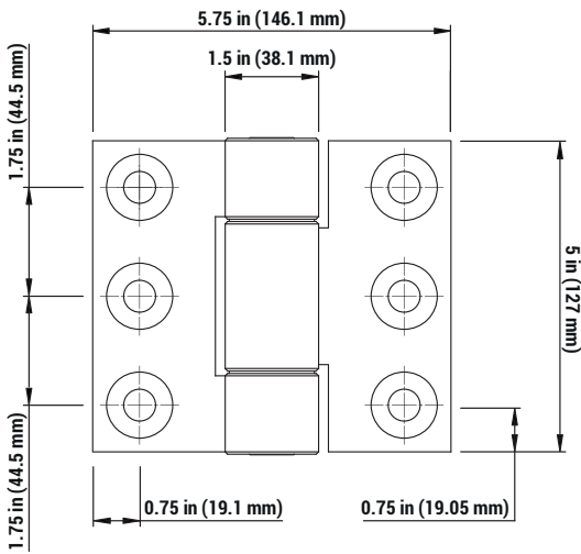
HT12 ELEVATION VIEW
